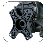
GR1-CPC-GCI Version Gear Reduction AR1639 with 1" Hollow Shaft, VDR50 Control Unit and 1 3/8" Splined Thru Shaft
