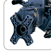
GR1-GCI/A1 Version Gear Reduction AR1639 with 1" Hollow Shaft, RM40 Control Unit and 1" Solid Keyed Thru Shaft
