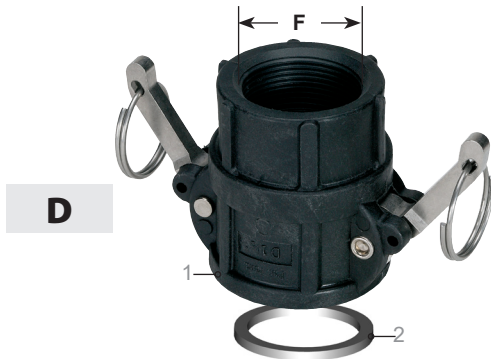
Female coupler » Female thread
